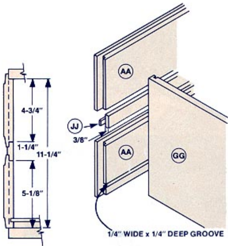
DETAIL OF FILE DRAWER ASSEMBLY
