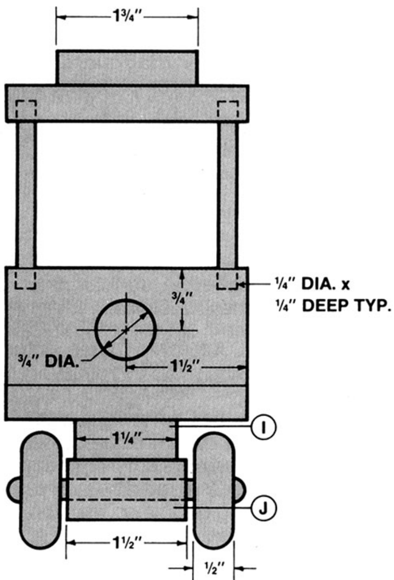
END VIEW
