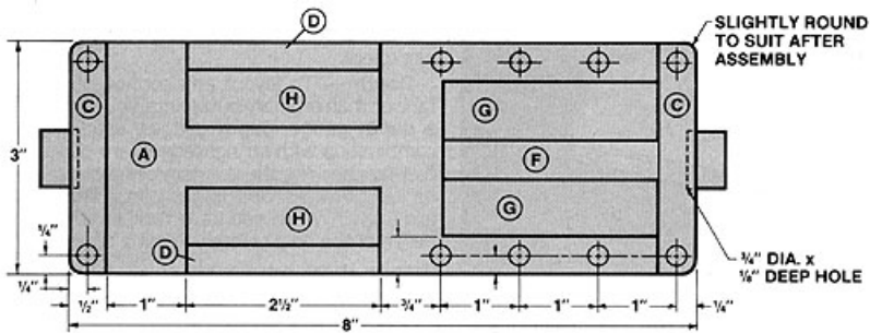
BASE LAYOUT
