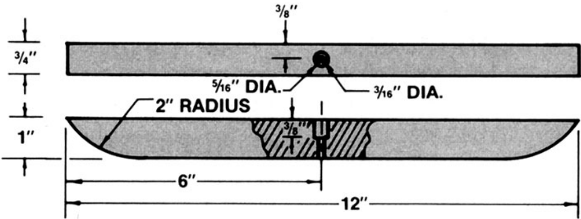
DROP LEAF SUPPORT COFFEE TABLE
