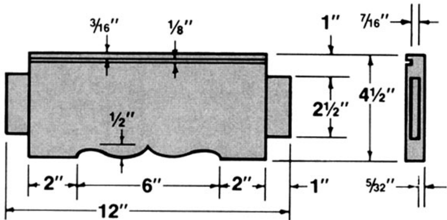
COFFEE TABLE END SKIRT AND TENON LAYOUT
