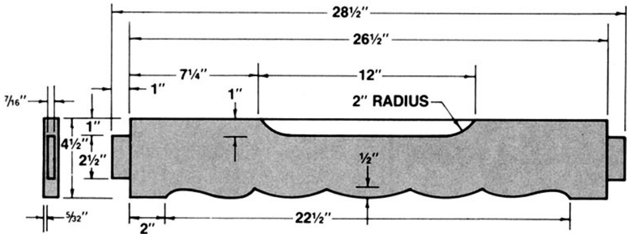
SIDE SKIRT AND TENON LAYOUT COFFEE TABLE
