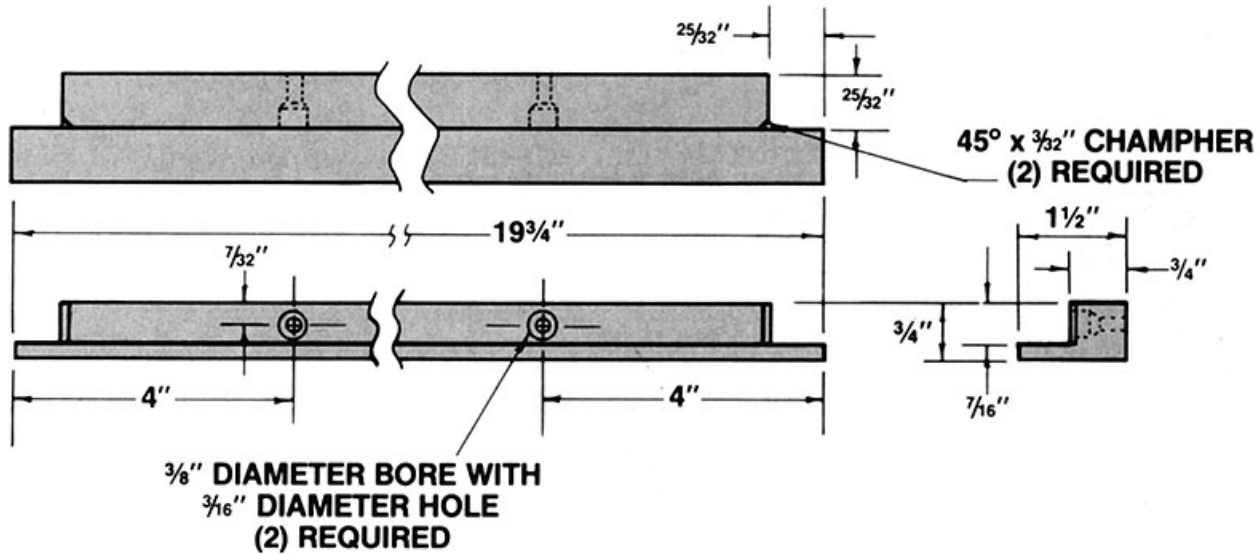
DRAWER GLIDE FOR CORNER AND END TABLE
