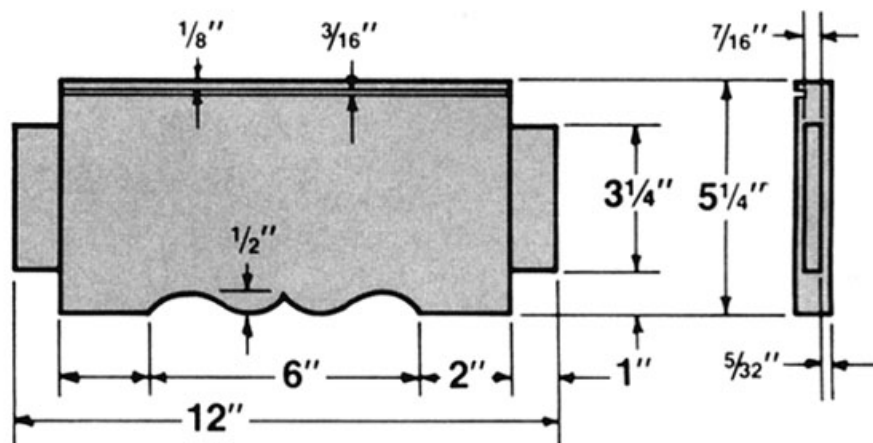
END TABLE END SKIRT AND TENON LAYOUT
