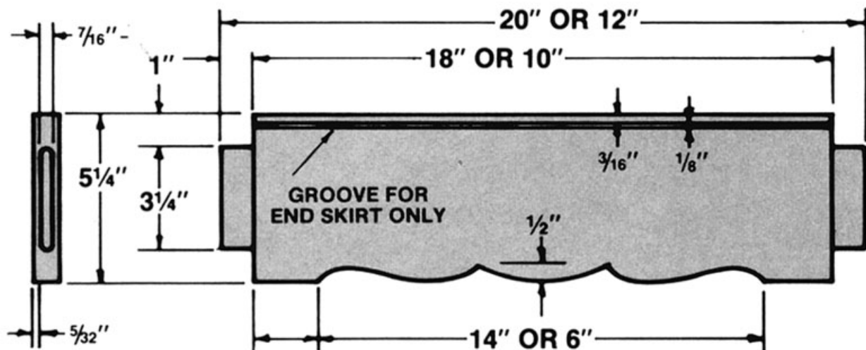
SIDE AND END SKIRT WITH TENON LAYOUT END TABLE AND CORNER TABLE
