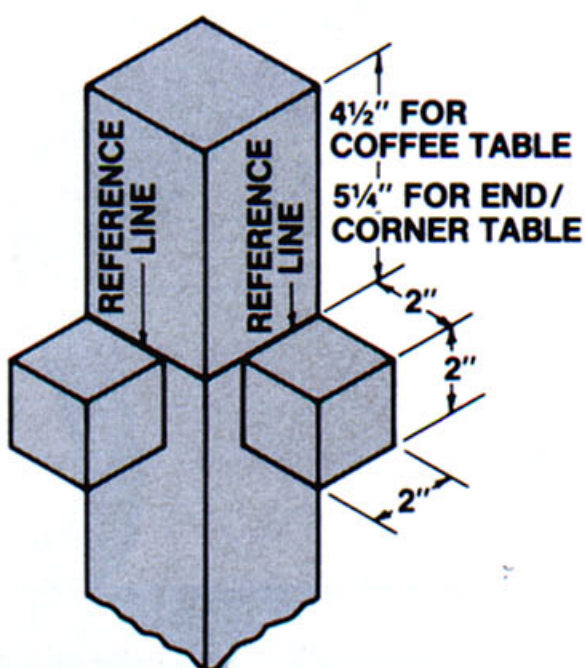
TRANSITION BLOCK LAYOUT FOR ALL TABLES
