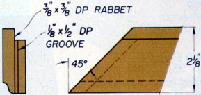
CORNER JOINT DETAIL
