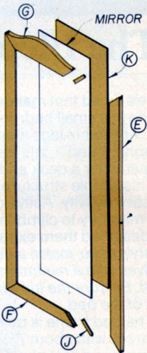
FRAME ASSEMBLY
