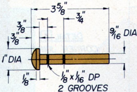
PIN LAYOUT
