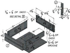
DRAWER ASSEMBLY
