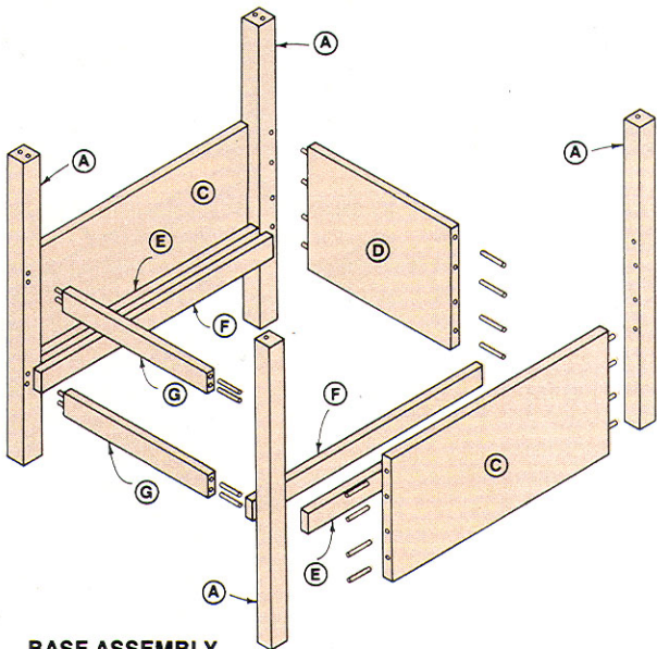
BASE ASSEMBLY
