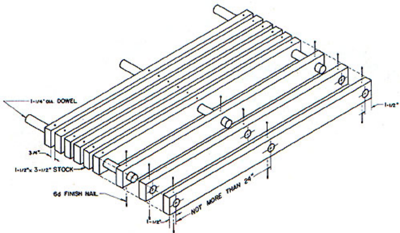
DUCKBOARD ASSEMBLY
