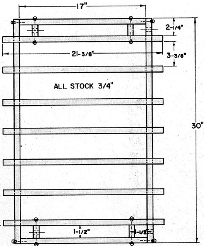
SHELF LAYOUT
