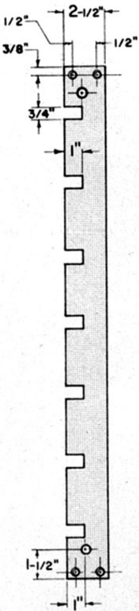
FRONT FRAME
