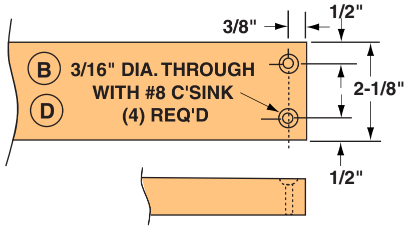
UPPER & LOWER BRACE END LAYOUT
