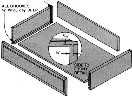
TYPICAL INSERT DRAWER CONSTRUCTION
