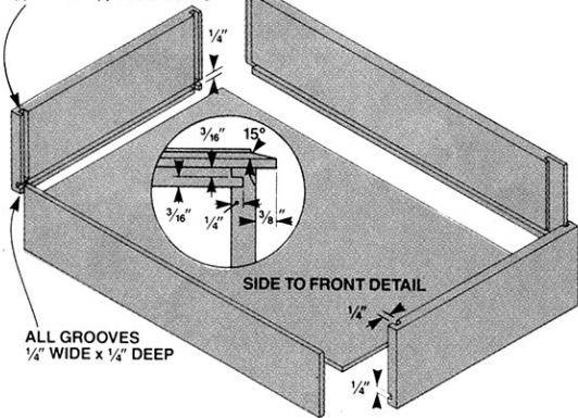
TYPICAL TOP DRAWER CONSTRUCTION
