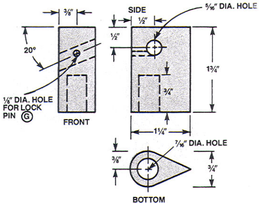
(F) SHOCK ABSORBER DETAIL
