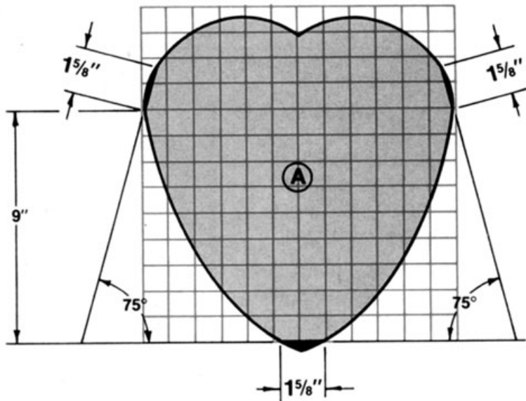
FIGURE 2 SHELF DESIGN
