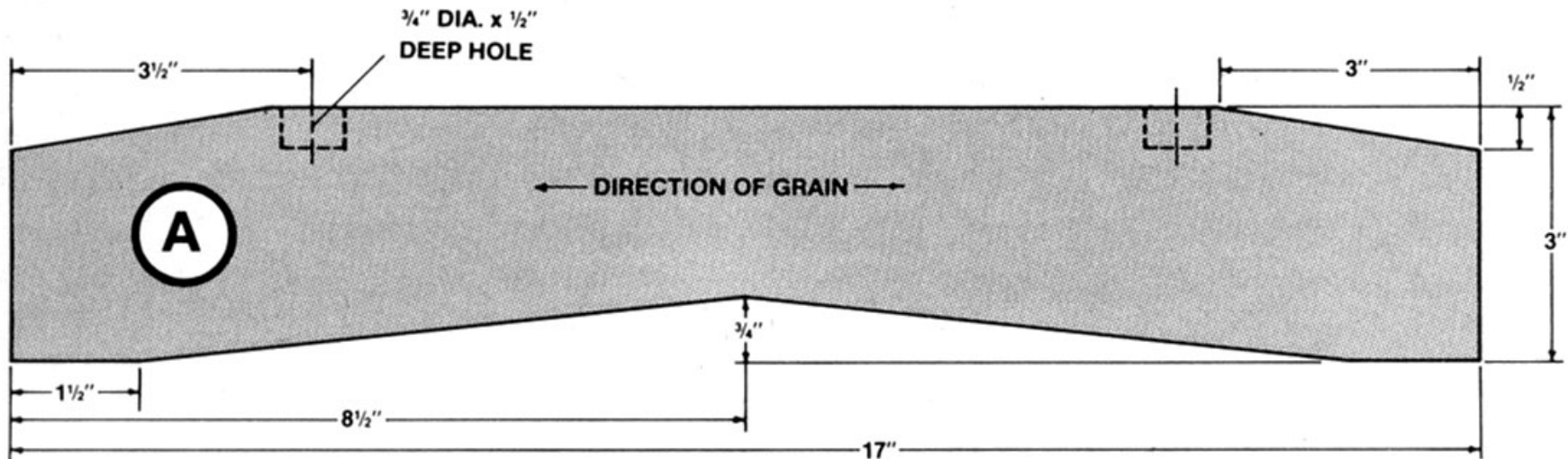
BASE (side view)
