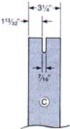
LEG SLOT LAYOUT
