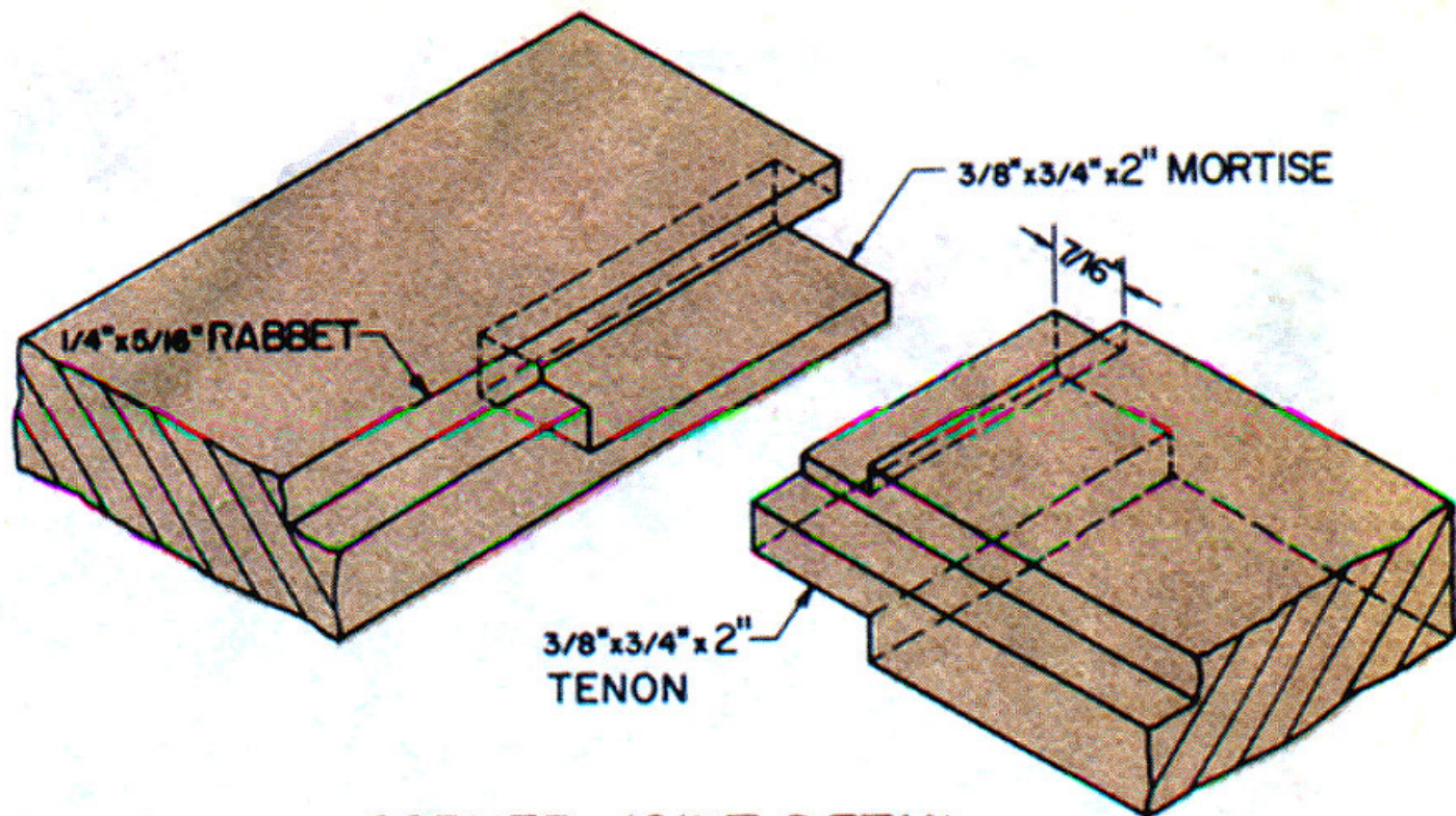
CORNER JOINT DETAIL
