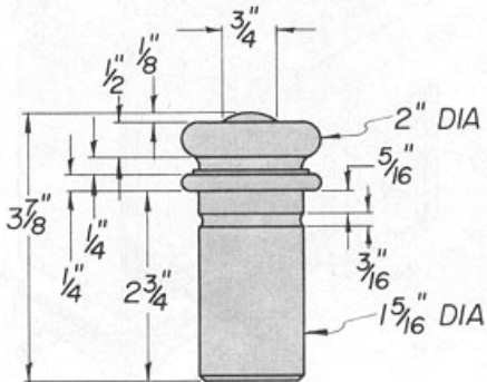
PIN LAYOUT
