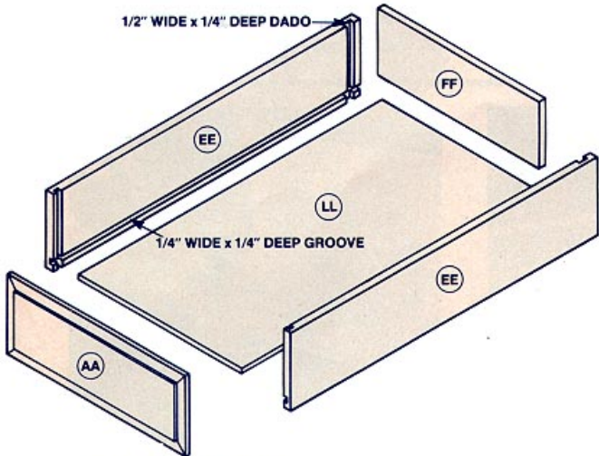
DRAWER ASSEMBLY
