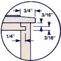
DRAWER DETAILS
